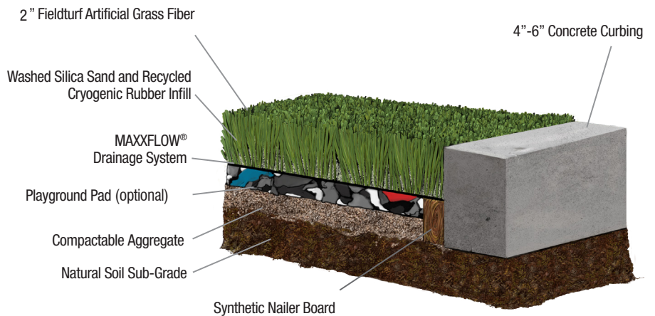
Edge Detail: Lumber or Nail Board 2"-4" Treated lumber or synthetic wood nailer board (not supplied by EasyTurf)
